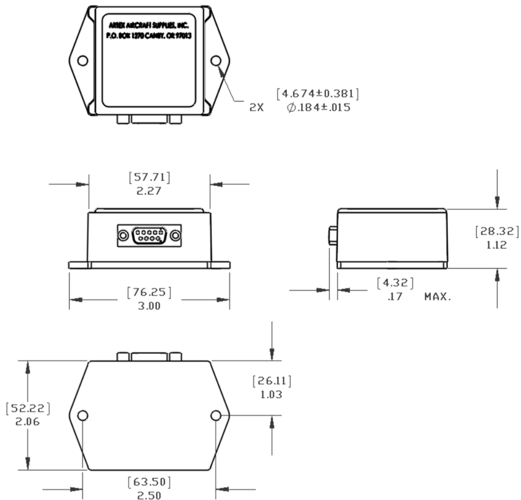
Figure 10: 453-0032 Interface
