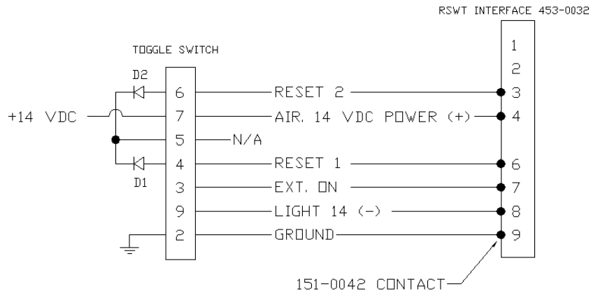
Figure 4: 453-0032 Wiring Diagram For 14 VDC Installation
