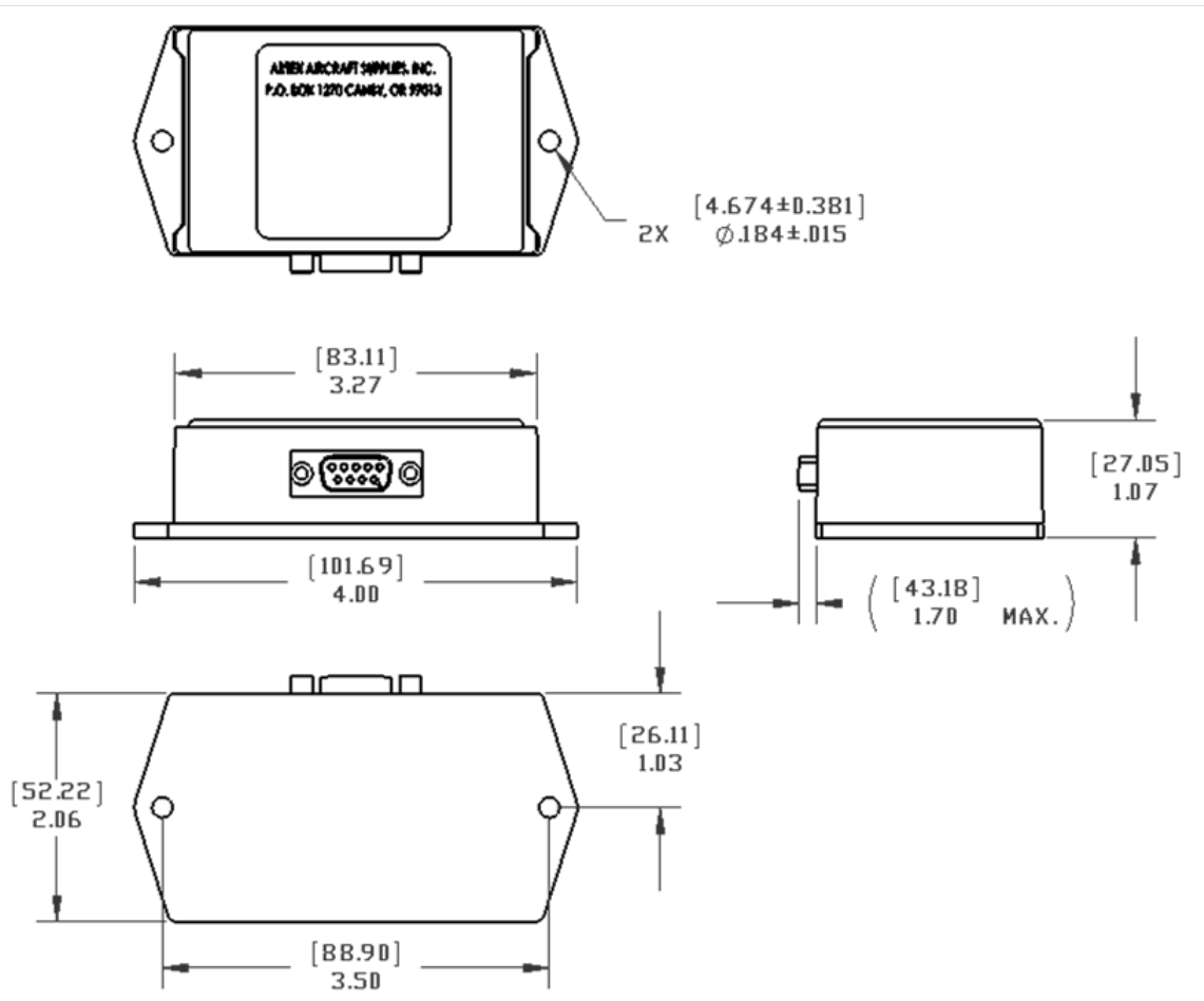
Figure 11: 453-0041 Interface
