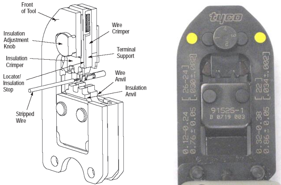
Figure 2: Tyco Crimping Tool
