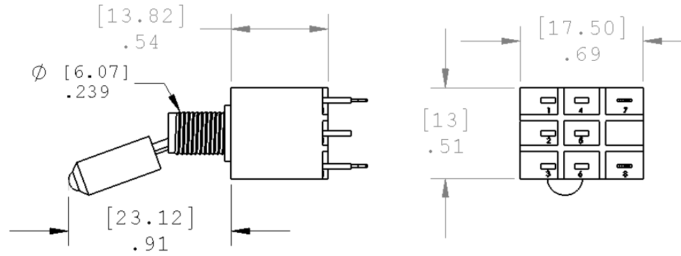
Figure 12: 140-3349 Toggle Switch
